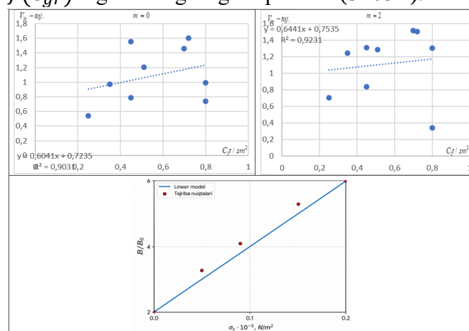
5-rasm. Birikishning o'zan kengligi yoyilishiga ta'siri v_{kr} = f(C_b) (tajriba).
