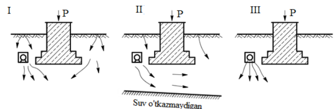
1-rasm. Poydevor asosining namlanish sxemasi:
