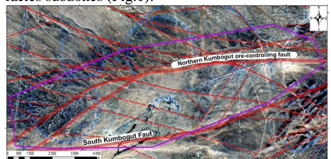
Fig.1. Results of preliminary space-structural interpretation of satellite imagery.
