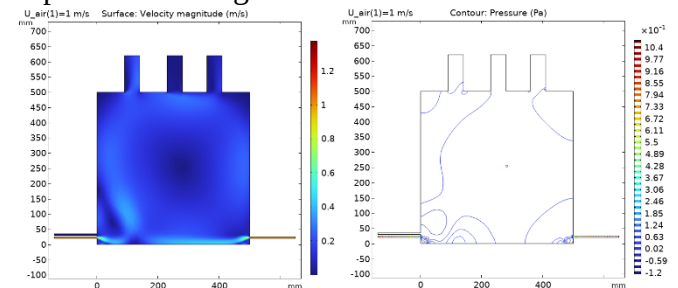
Fig.2. Aerodynamic behavior in the combustion chamber when the inlet air flow velocity is 1 m/s.
