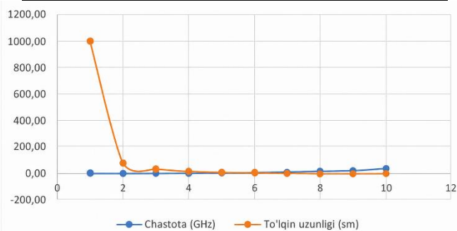
Diapazon nomi Chastota To'liq uzunligi VHF 30–300 MHz 10–1 m P-band 280–390 MHz 107–77 sm UHF 300 MHz – 1 GHz 100–30 sm L-band 1–2 GHz 30–15 sm S-band 2–4 GHz 15–7.5 sm C-band 4–8 GHz 7.5–3.75 sm X-band 8–12.5 GHz 3.75–2.40 sm Ku-band 8–12.5 GHz 2.40–1.67 sm K-band 18–25 GHz 1.67–1.18 sm Ka-band 25–40 GHz 1.18–0.75 sm
