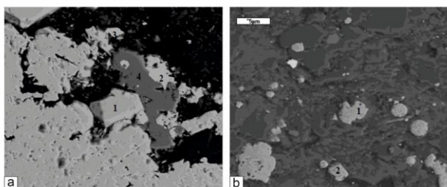
4-rasm. Sulfidli va aksessor minerallarning o'zaro o'sishmalari:
