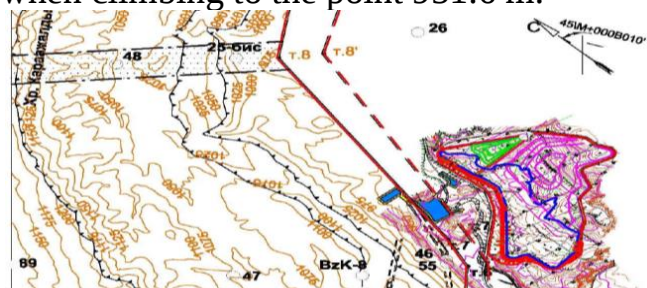
Figure 1. The scheme of the location of the salt dump, which was mined as a result of the passage of mine solder from the salt layer for the construction of the mine, and the dump consisting of salt waste from the DPP.
