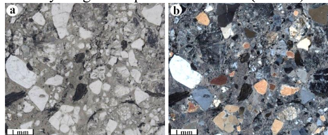
4-rasm. Andezidatsit tarkibli tuffizit (inyeksion tuf).
