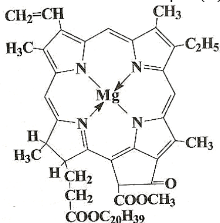
1-rasm Xlorofill-ligant.
