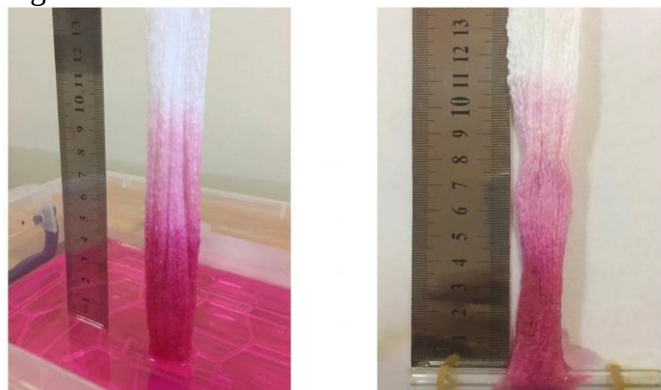
Fig.3. The process of testing the capillary properties of fabrics.
