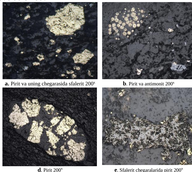
2-rasm. a-b-alevrolit, d-e-uglerodli slanes.
