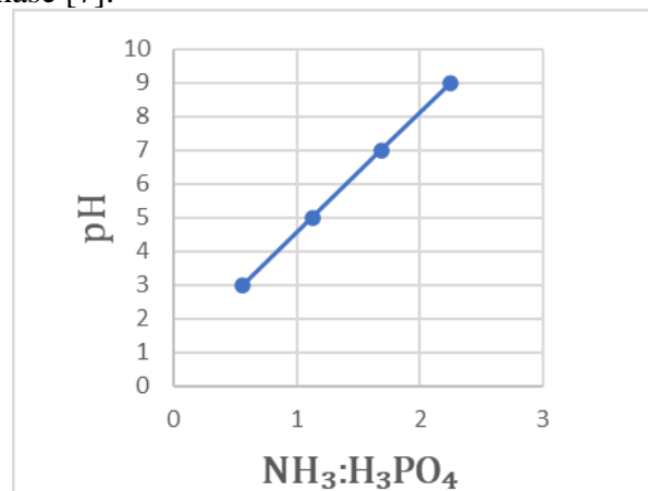
Figure 1. The relationship between pH value and the molar ratio of NH 3 :H 3 PO 4 in saturated solutions of ammonium phosphates at temperatures of 65–75°C.
